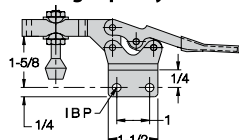
CL-451-HTC Straight Base
