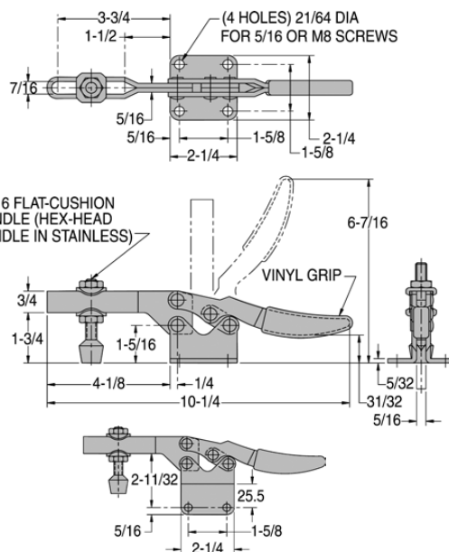
CL-551-HTC Straight Base
